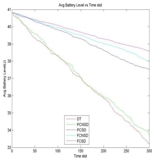
Fig 10 : Average battery level \sum_k B_k / |K| of the MTs over time slot
