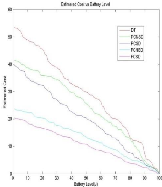
Fig 9 : Expected cost of multiple source MTs versus battery level under different mode of transaction
