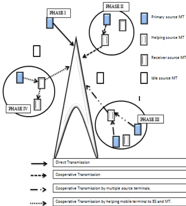
Fig.1 : Cooperative communication with four phases
