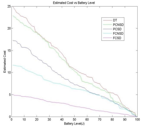
Fig 7. Expected cost for single source MT versus battery level under different mode of transaction
